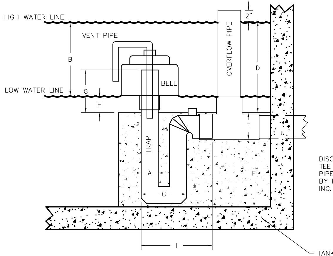
APPROXIMATE DIMENSIONS IN INCHES
