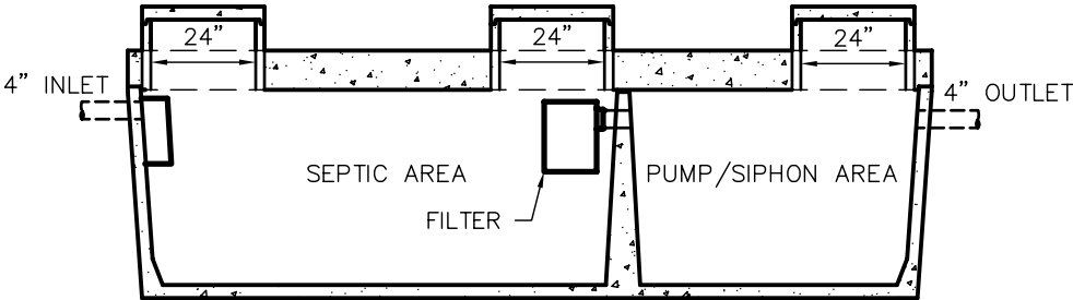
COMBINATION TANK
