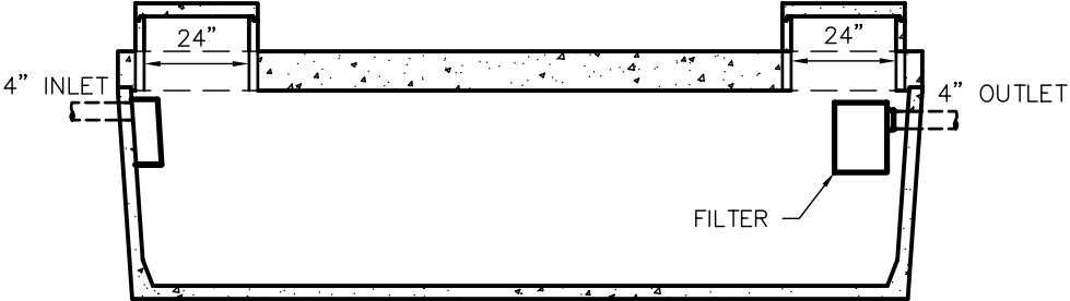
SEPTIC TANK
